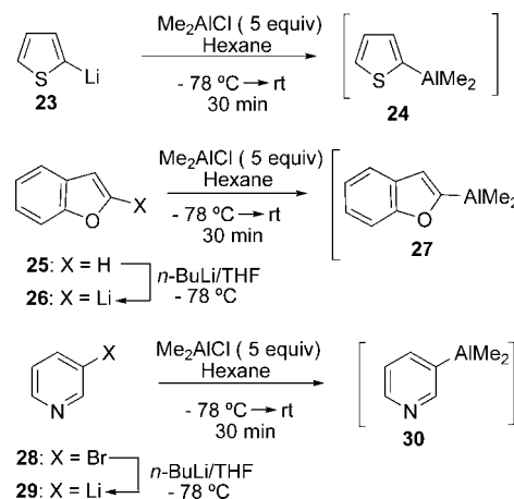
SCHEME 7. Preparation of Dimethyl Heteroaryl Aluminum Reagents 24 , 27 , and 30
